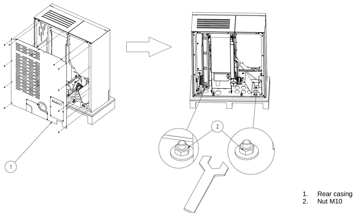
Fig. № 3 Dismantling the fireplace from the pallet
